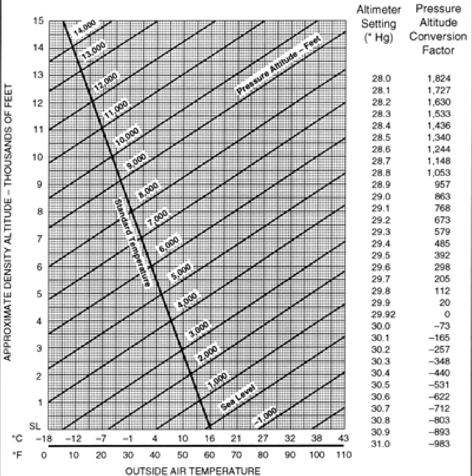
FIGURE 8.—Density Altitude Chart.
